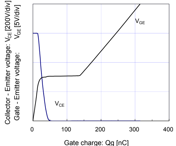
Dynamic gate charge (typ.) V CC =600V, I c =50A, T j = 25°C
